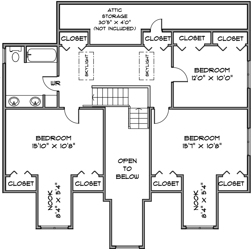
UPPER LEVEL 1000 SQ. FT.
