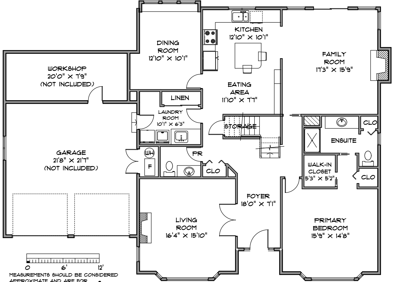
MAIN LEVEL 1833 SQ. FT.
