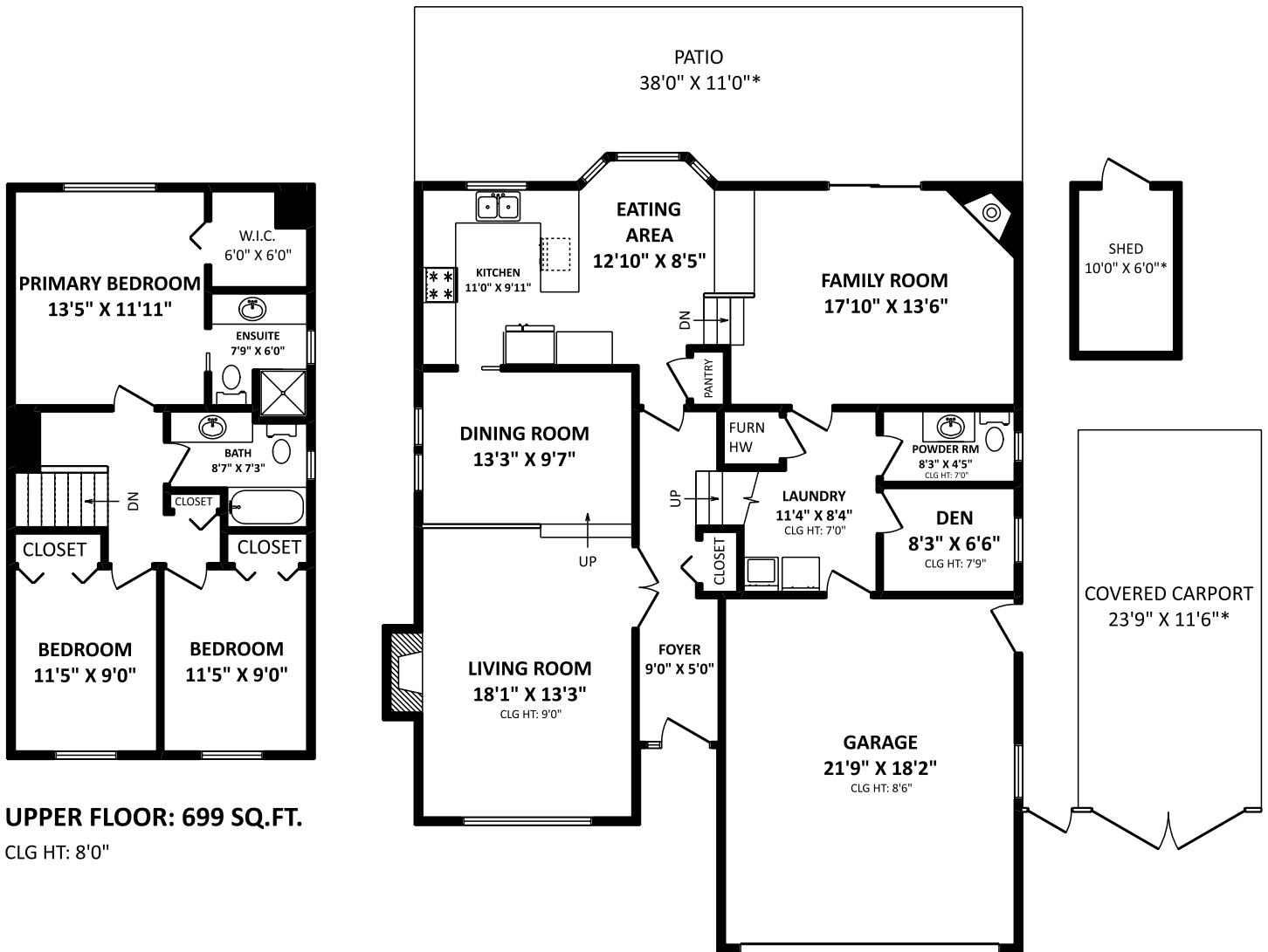
MAIN FLOOR: 774 SQ.FT. CLG HT: 8'0", U.N.O.
