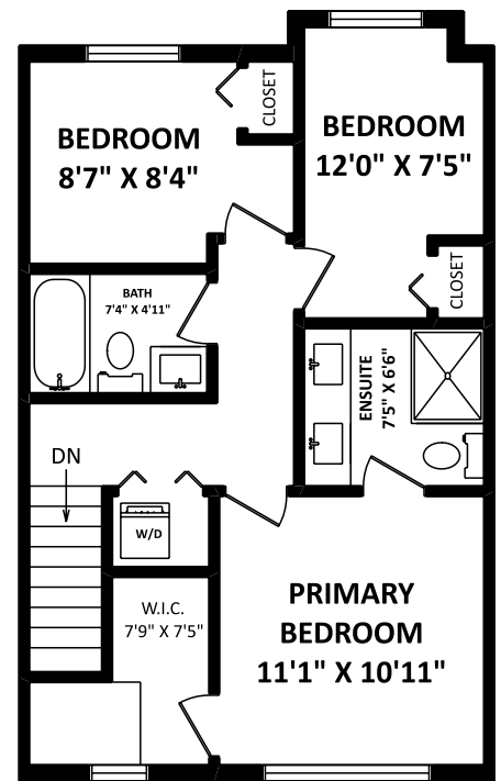
UPPER FLOOR: 590 SQ.FT.
