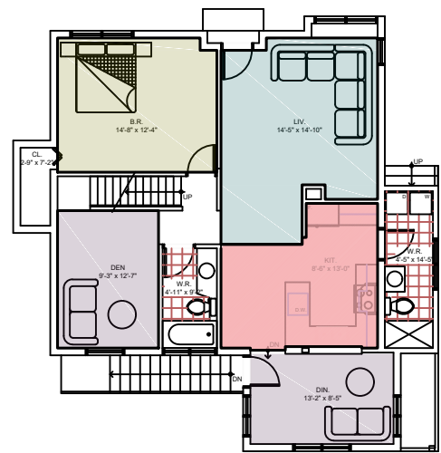
LEVEL 2 FLOOR PLAN 1156.33 SF
