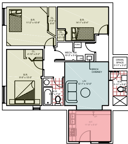
LEVEL 1 FLOOR PLAN 1090.81 SF
