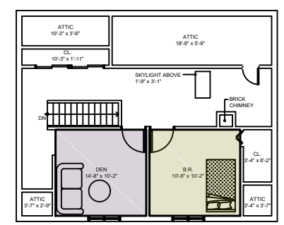
LEVEL 3 FLOOR PLAN 767.23 SF
