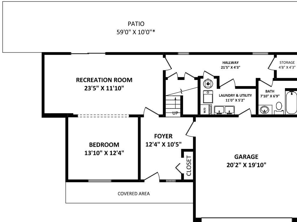
LOWER FLOOR: 968 SQ.FT.
