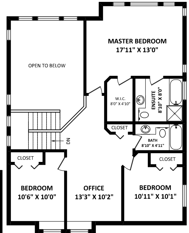
UPPER FLOOR: 1071 SQ.FT.
