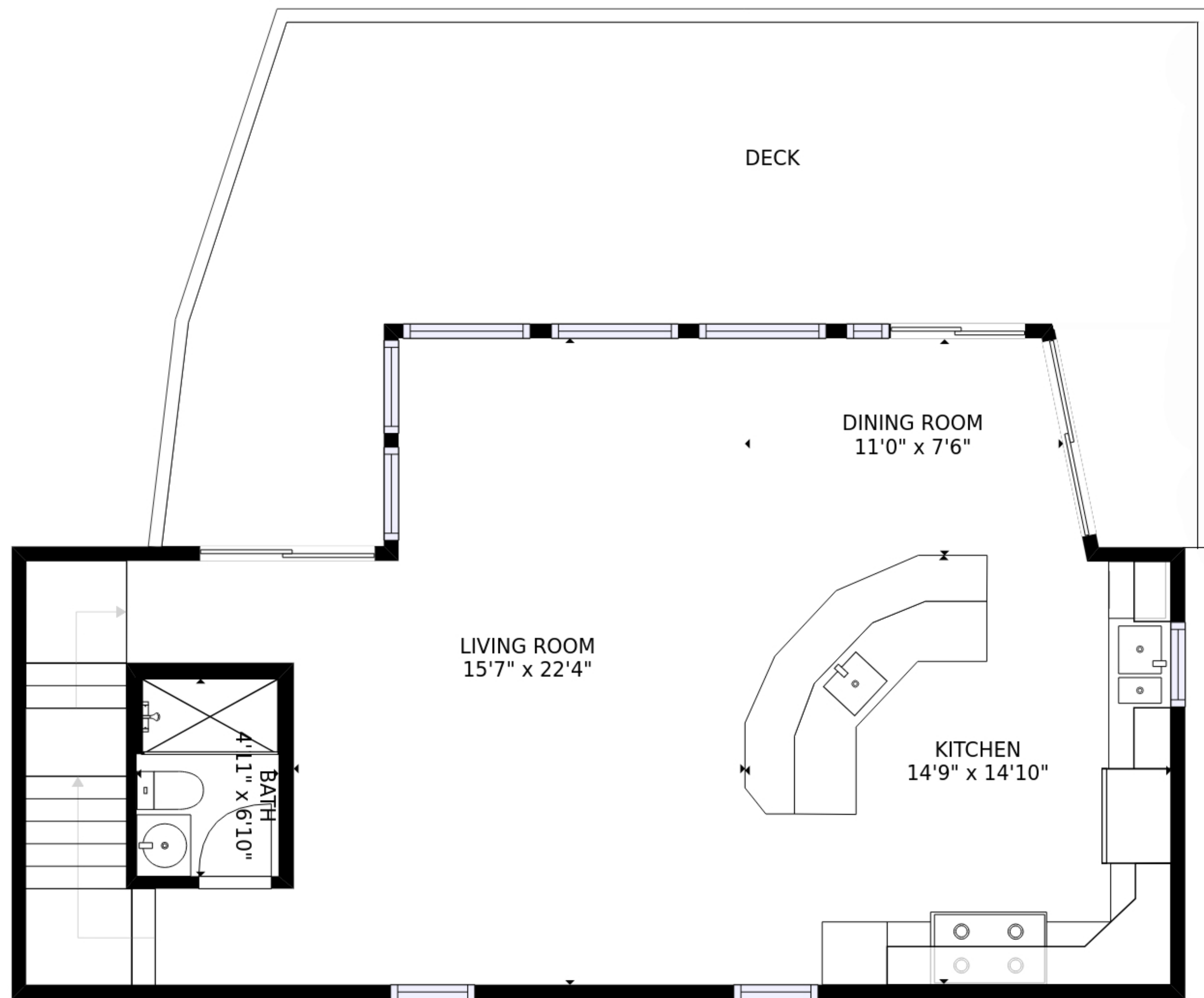
FLOOR 2
