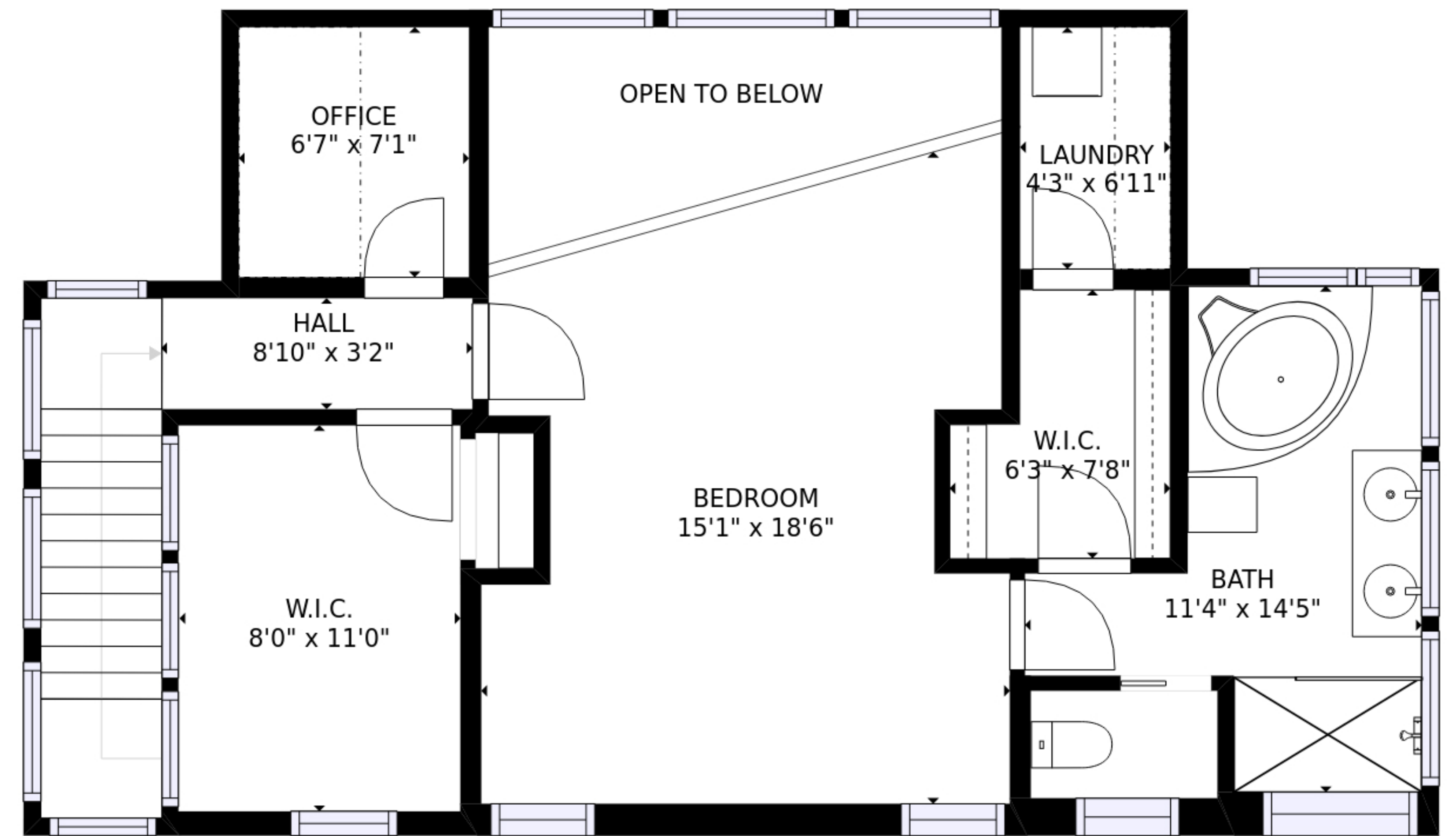
FLOOR 3
