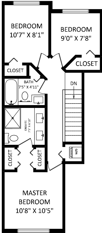
UPPER FLOOR: 609 SQ.FT.
