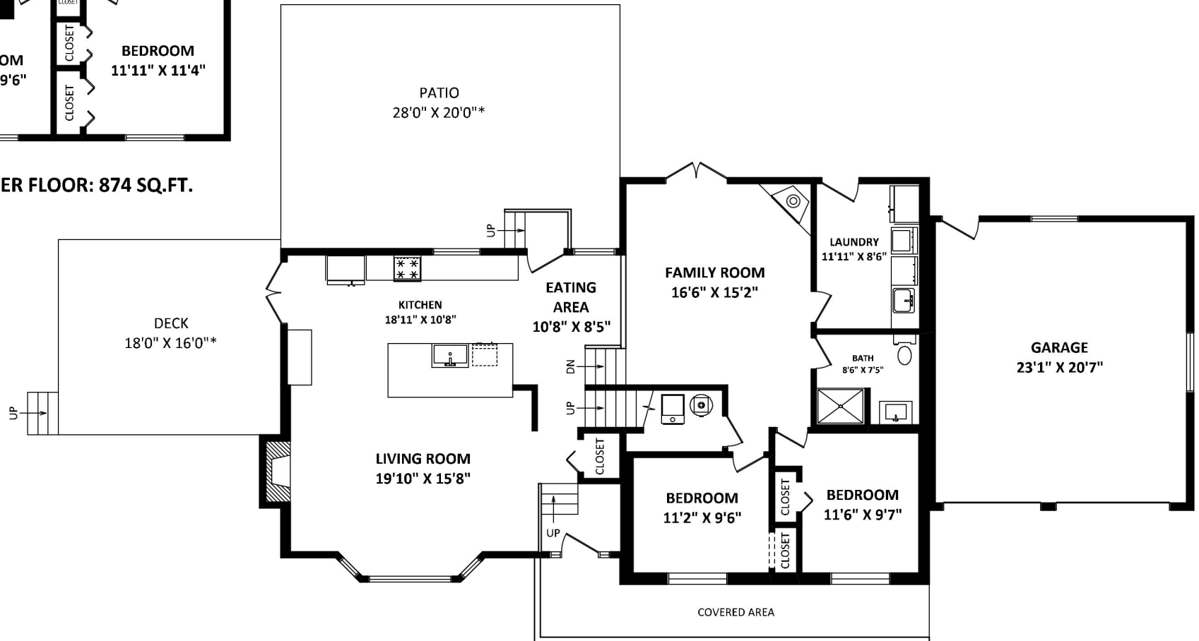
MAIN FLOOR: 732 SQ.FT. LOWER FLOOR: 848 SQ.FT.
