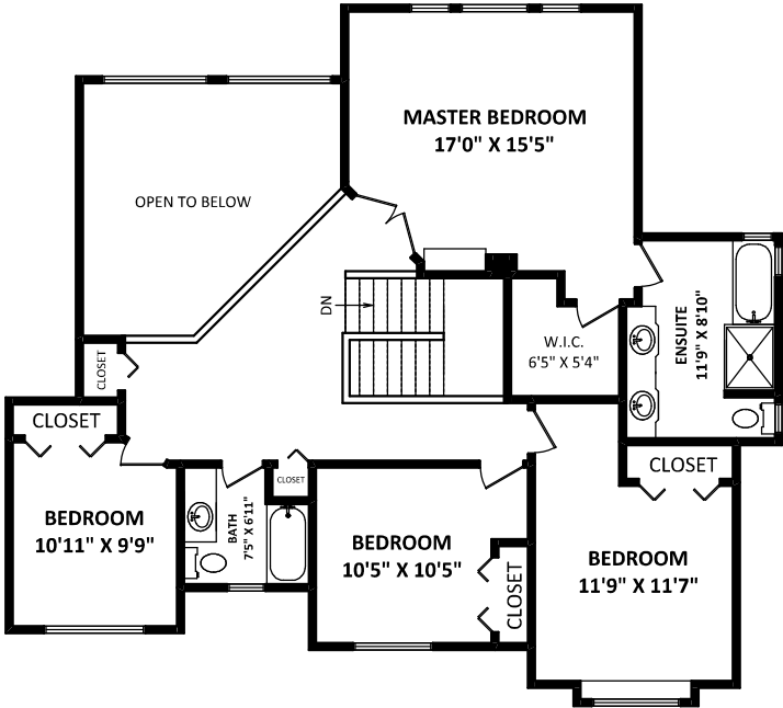
UPPER FLOOR: 1246 SQ.FT.
