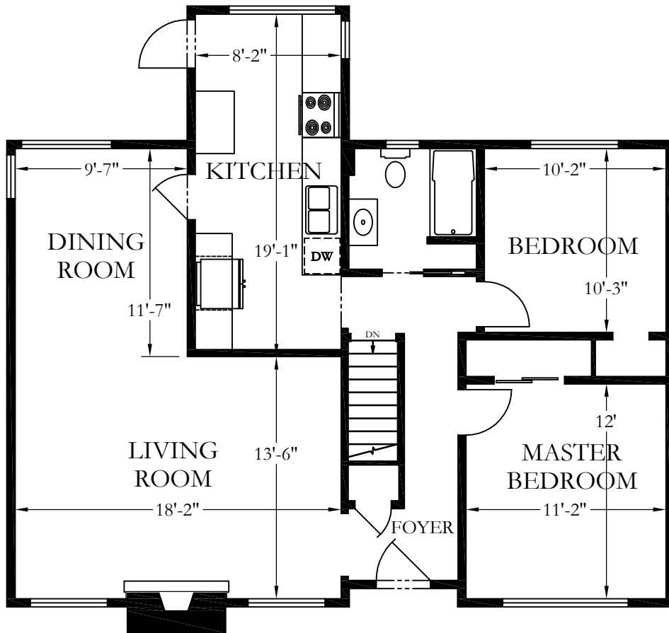
MAIN FLOOR
