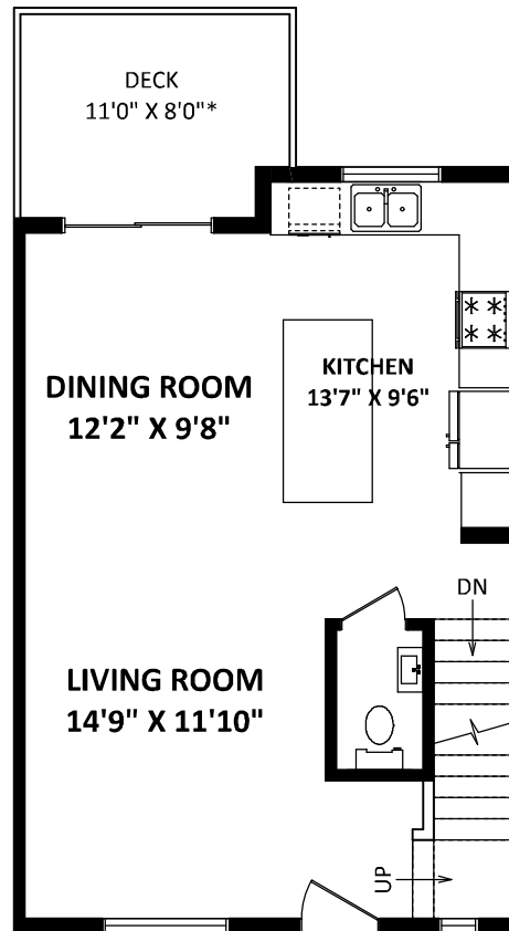
MAIN FLOOR: 570 SQ.FT.
