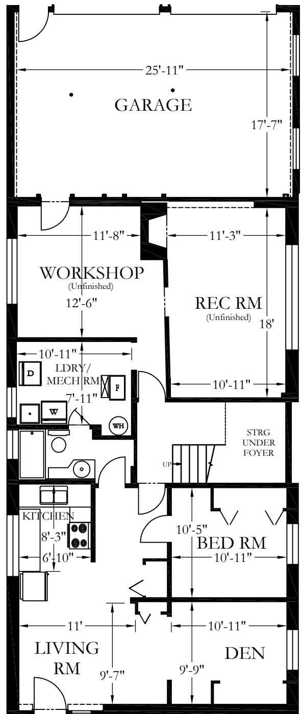
LOWER FLOOR
