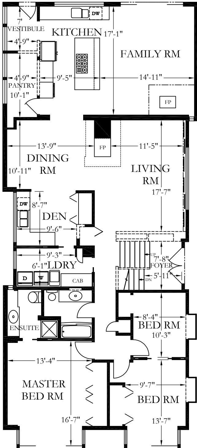
UPPER FLOOR
