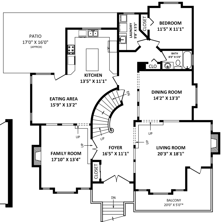
MAIN FLOOR: 1908 SQ.FT.
