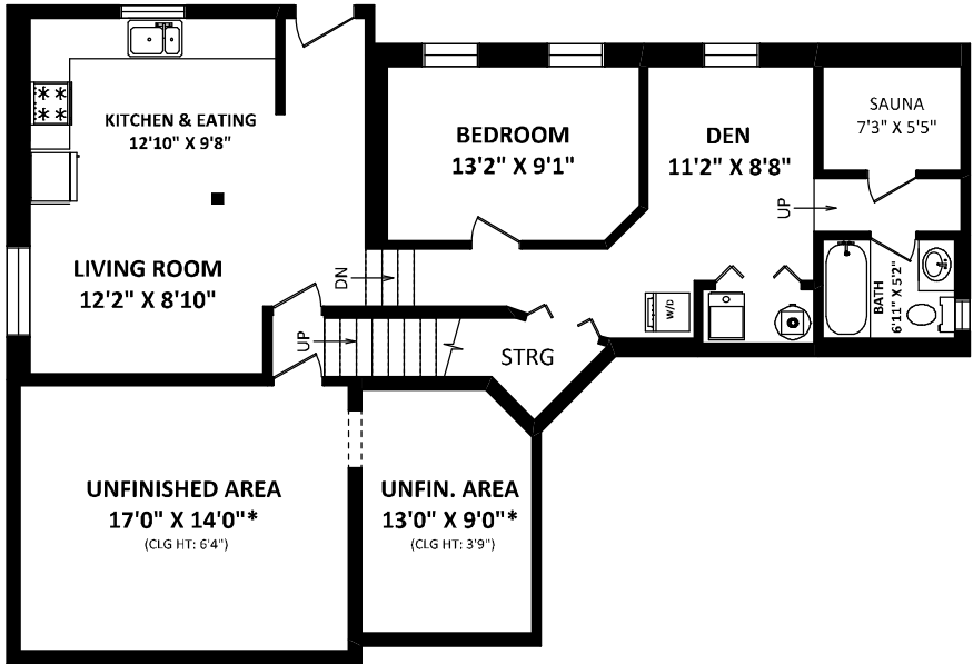
BOTTOM FLOOR: 906 SQ.FT.
