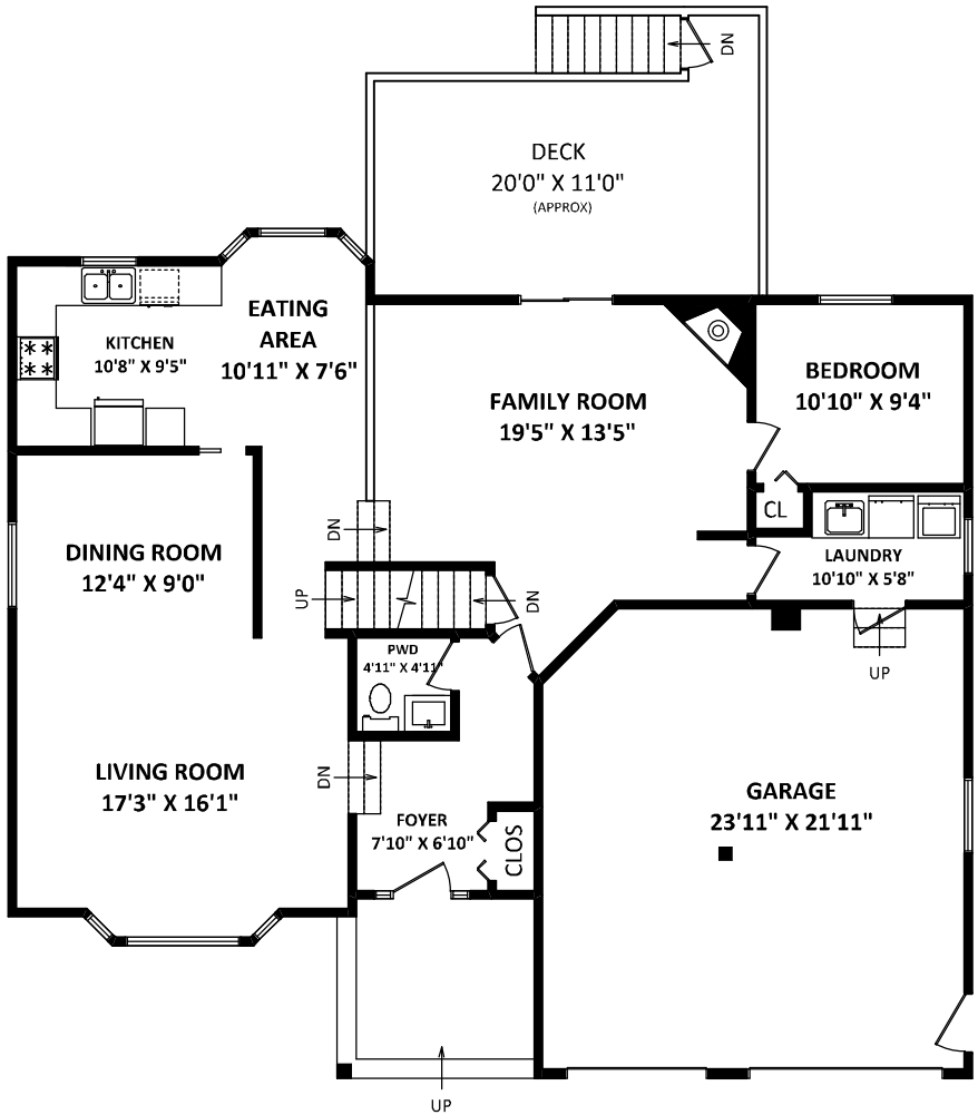
MAIN FLOOR: 792 SQ.FT. LOWER FLOOR: 526 SQ.FT.
