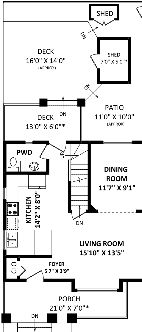
MAIN FLOOR: 607 SQ.FT.
