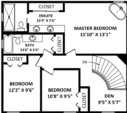
UPPER FLOOR: 932 SQ.FT.
