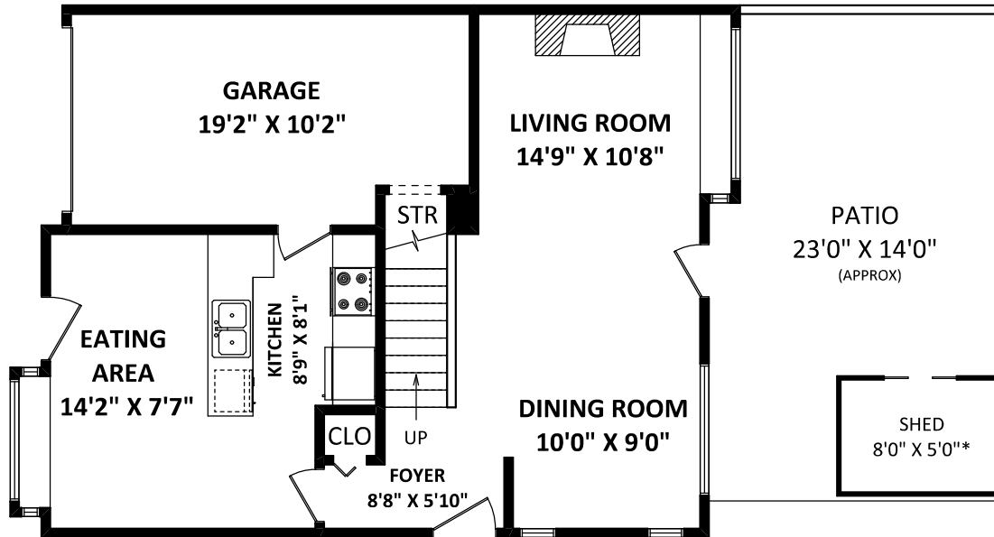
MAIN FLOOR: 584 SQ.FT.
