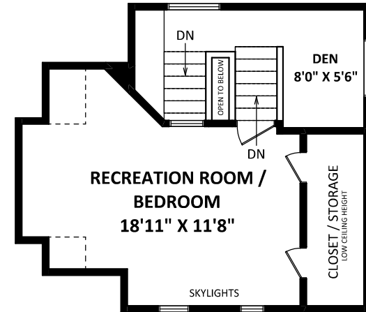
TOP FLOOR: 366 SQ.FT.
