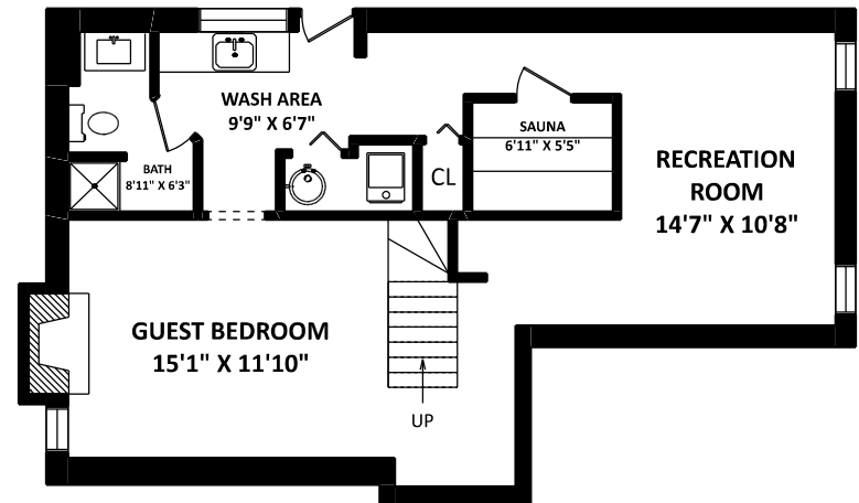
LOWER FLOOR: 850 SQ.FT.
