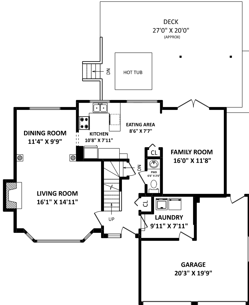
MAIN FLOOR: 981 SQ.FT.
