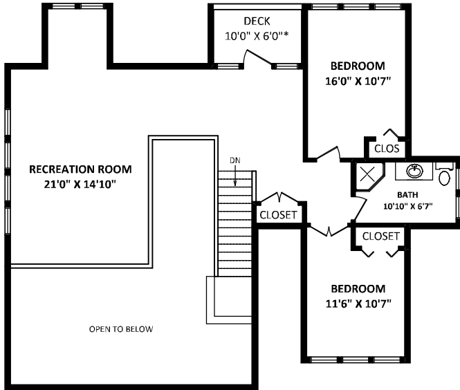
UPPER FLOOR: 1167 SQ.FT.
