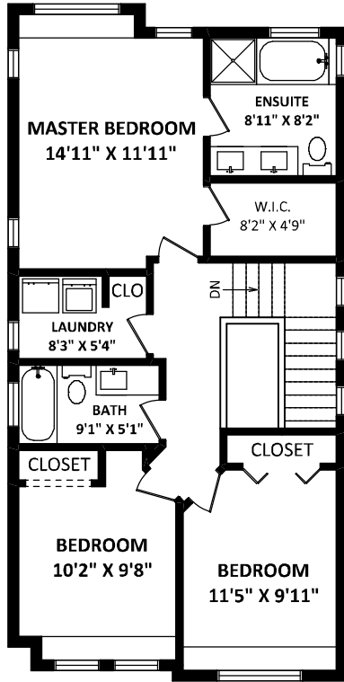
UPPER FLOOR: 856 SQ.FT.
