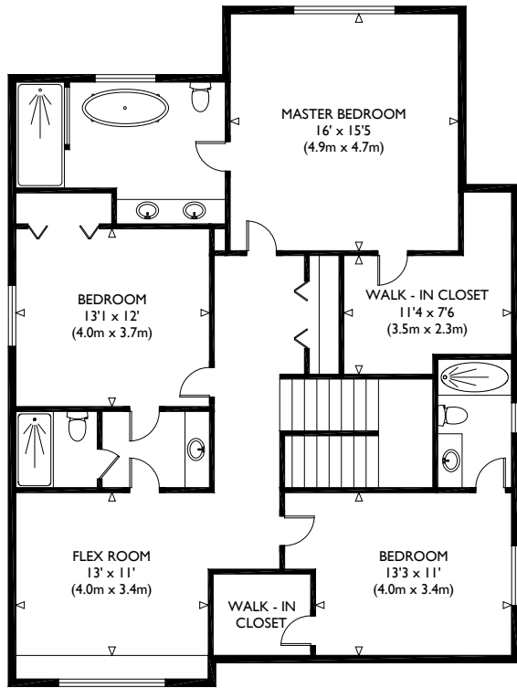
UPPER FLOOR GROSS INTERNAL FLOOR AREA 1323 SQ FT
