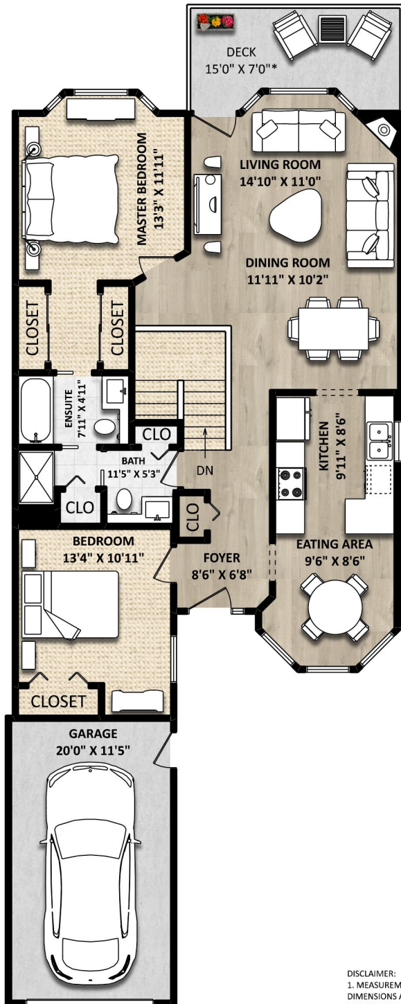
MAIN FLOOR: 1136 SQ.FT.
