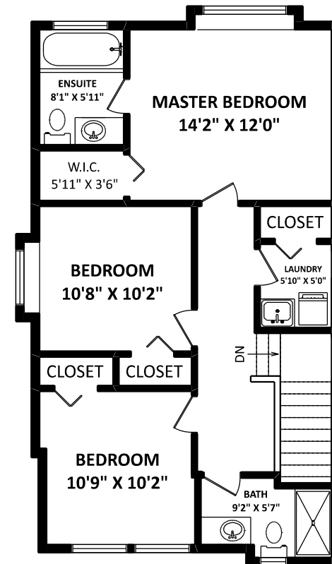
UPPER FLOOR: 815 SQ.FT.
