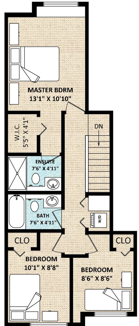
UPPER FLOOR: 638 SQ.FT.
