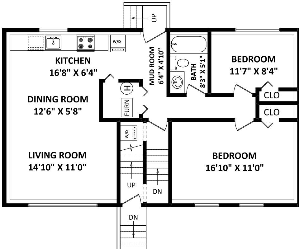
LOWER FLOOR: 959 SQ.FT.
