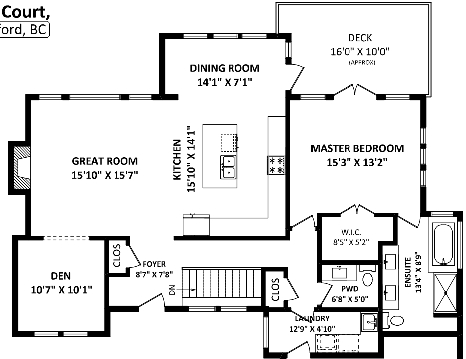
MAIN FLOOR: 1476 SQ.FT.
