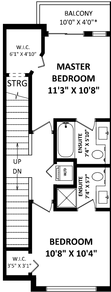
LOWER FLOOR: 530 SQ.FT.
