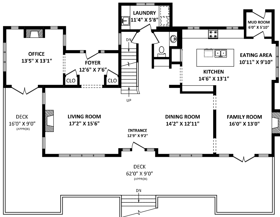
MAIN FLOOR: 1793 SQ.FT.
