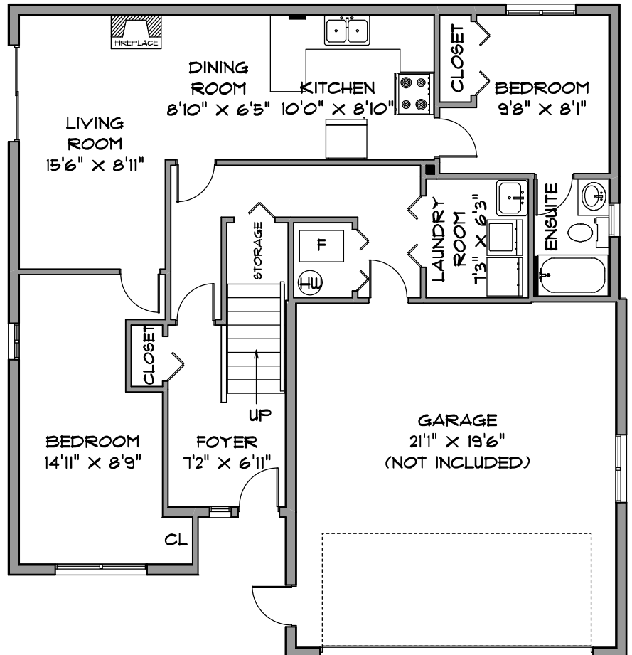
LOWER LEVEL 952 SQ.FT.
