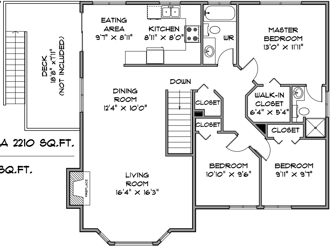
MAIN LEVEL 1248 SQ.FT.
