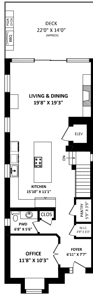
MAIN TOP FLOOR (4): 1145 SQ.FT.
