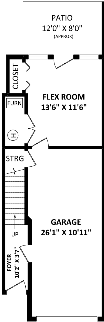
LOWER FLOOR: 48 SQ.FT. FLEX ROOM: 223 SQ.FT.
