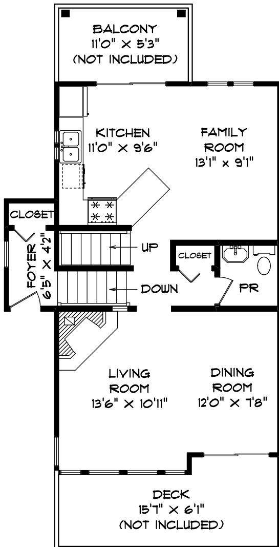
MAIN LEVEL 678 SQ.FT.
