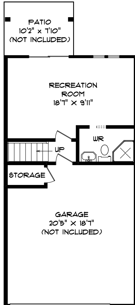
LOWER LEVEL 319 SQ.FT.
