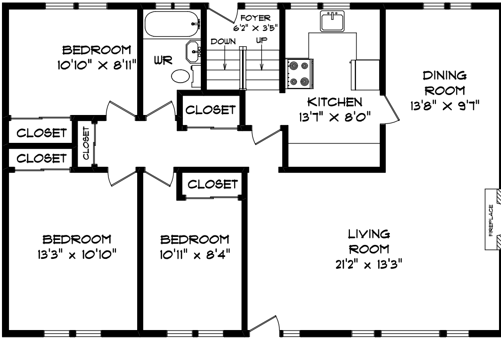
MAIN LEVEL 1193 SQUARE FEET
