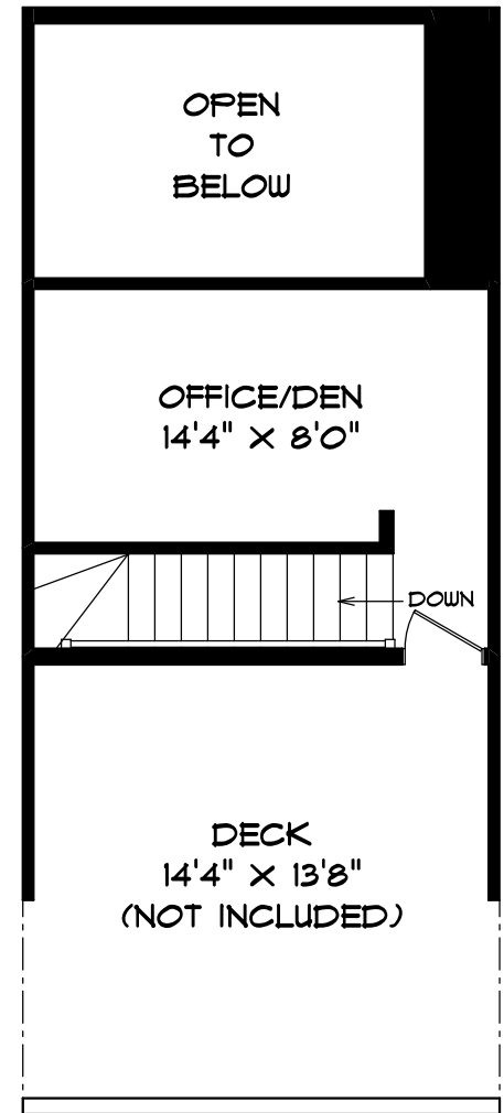
UPPER LEVEL 183 SQUARE FEET
